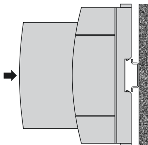
Fig. 5. Mounting on top-hat rail 35 × 15 or 35 × 7.5 mm.
