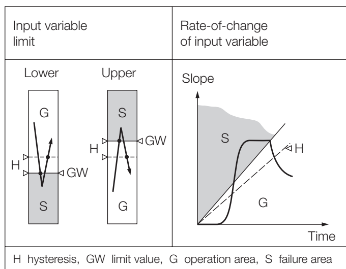
Fig. 5. Switching function according to limit monitored.
