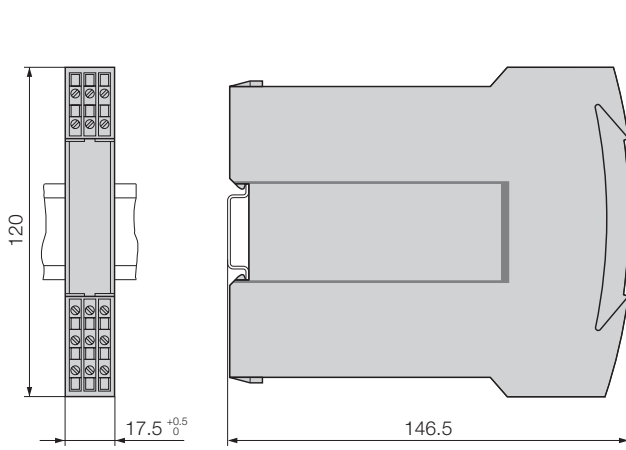
Fig. 4. SINEAX TV 808 in housing S17 clipped onto a top-hat rail (35 x 15 mm or 35 x 7.5 mm, acc. to EN 50 022).
