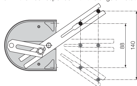
Fig. 4. Operating lever set for maximum operating angle.
